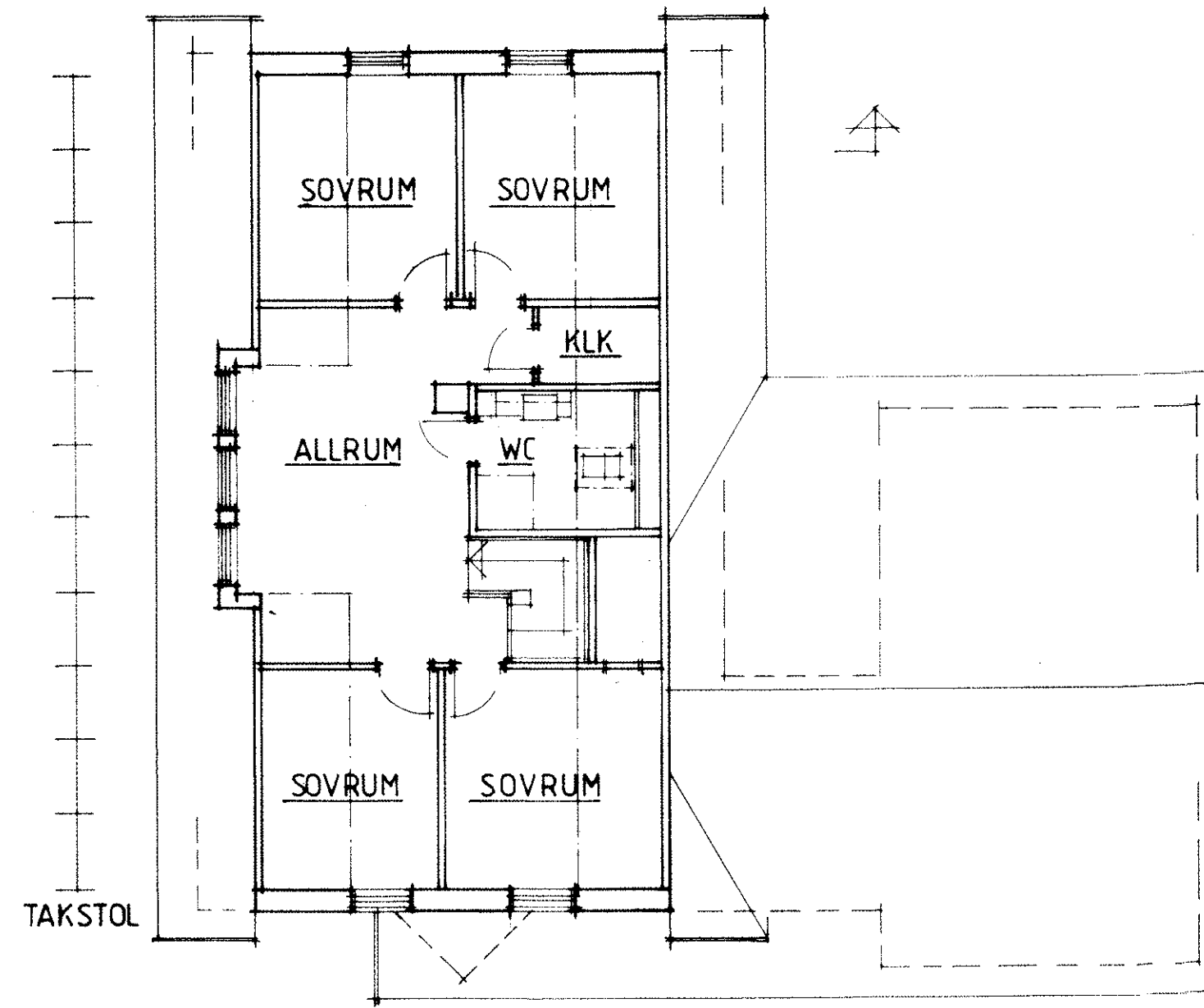
OVANPLAN
