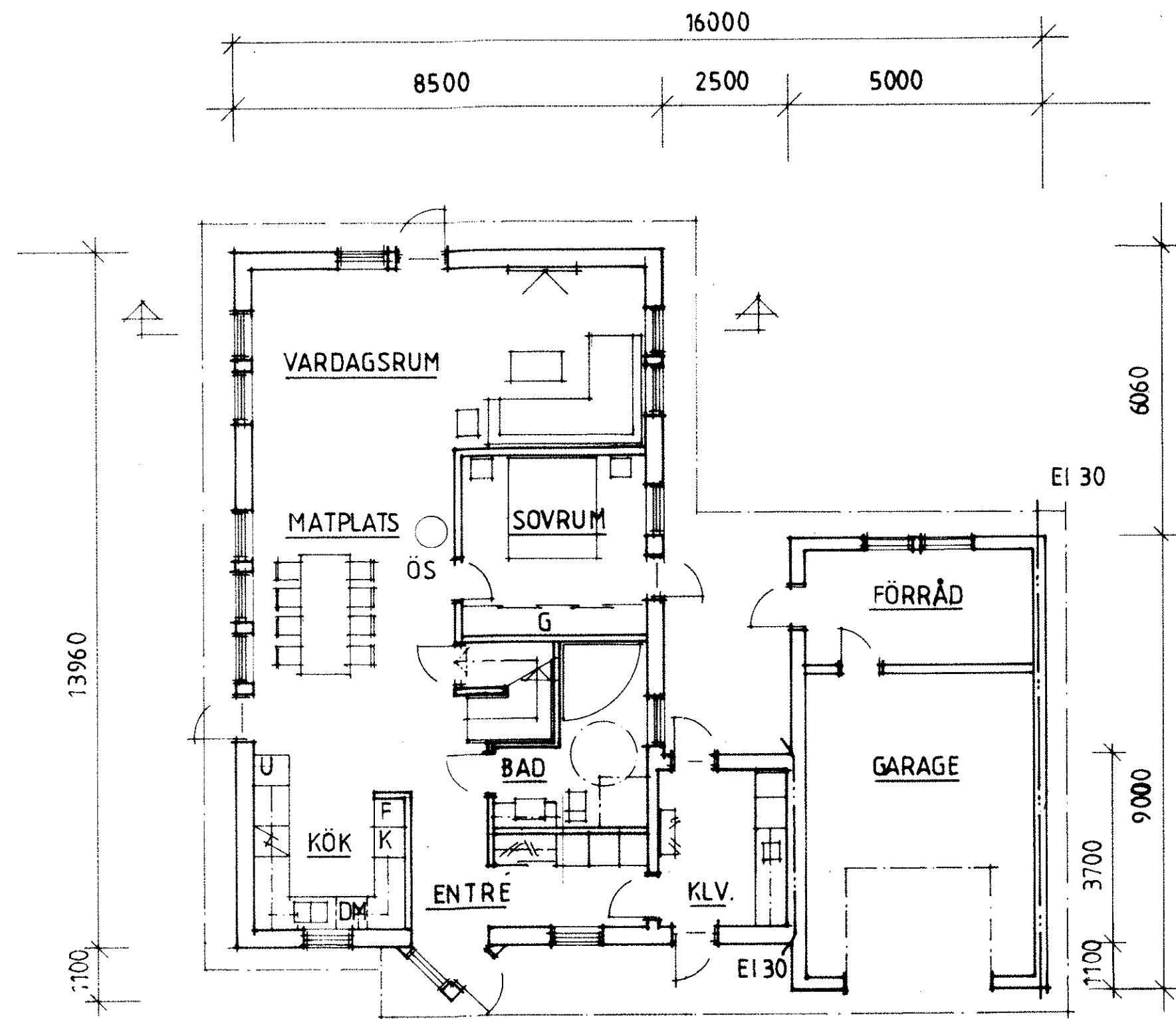
BOTTENPLAN
